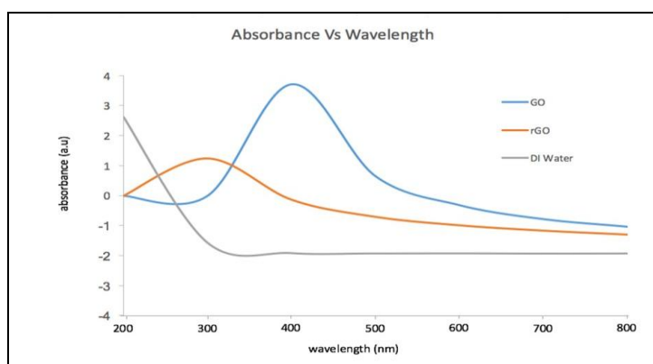
Figure 3. Uv-Vis graph of GO and rGO solution.
